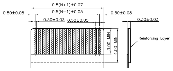
RECOMMENDED FFC DIM RECOMMENDED FFC DIM
