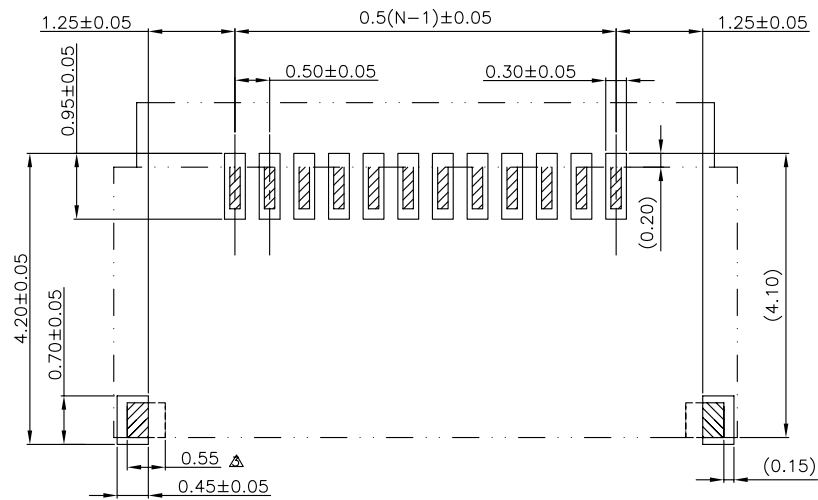
APPLICABLE P.C.B DIMENSION(REF.)
