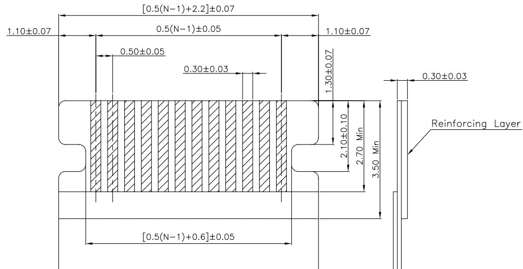
APPLICABLE F.P.C DIMENSION(REF.)
